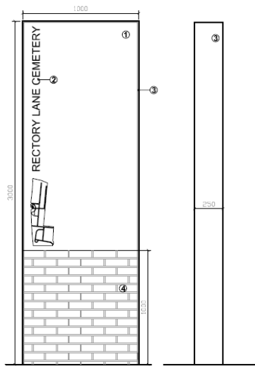
1:20 Monolith Sign Elevations @ A3
